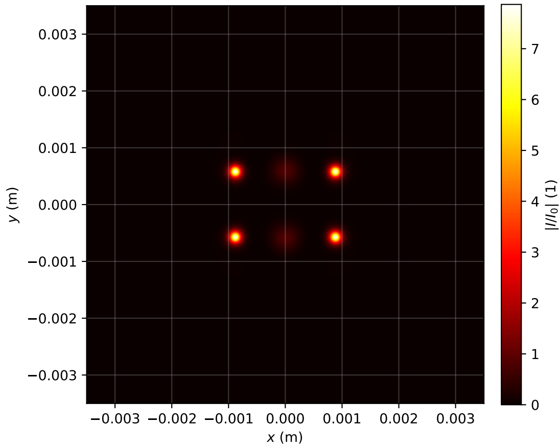
Intensity profile I(x, y, z = 0.955)/I_0 , P_{in}=5.0P_{cr} , artificial time
